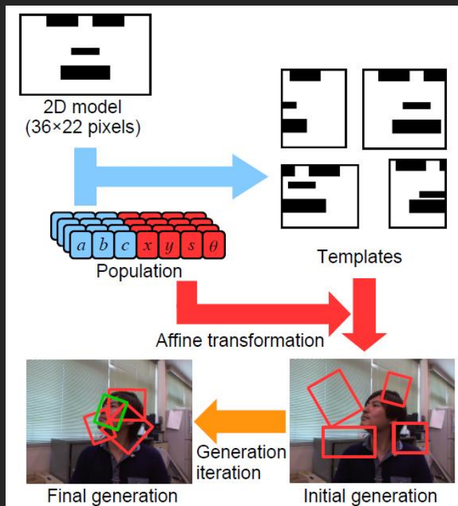
Outline of the proposed method
